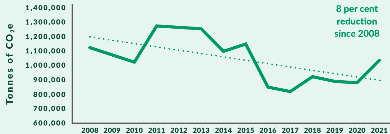
FIGURE 1. FOREST SUPPLY CHAIN SCOPE 1 & 2 EMISSIONS SINCE 2008 1
