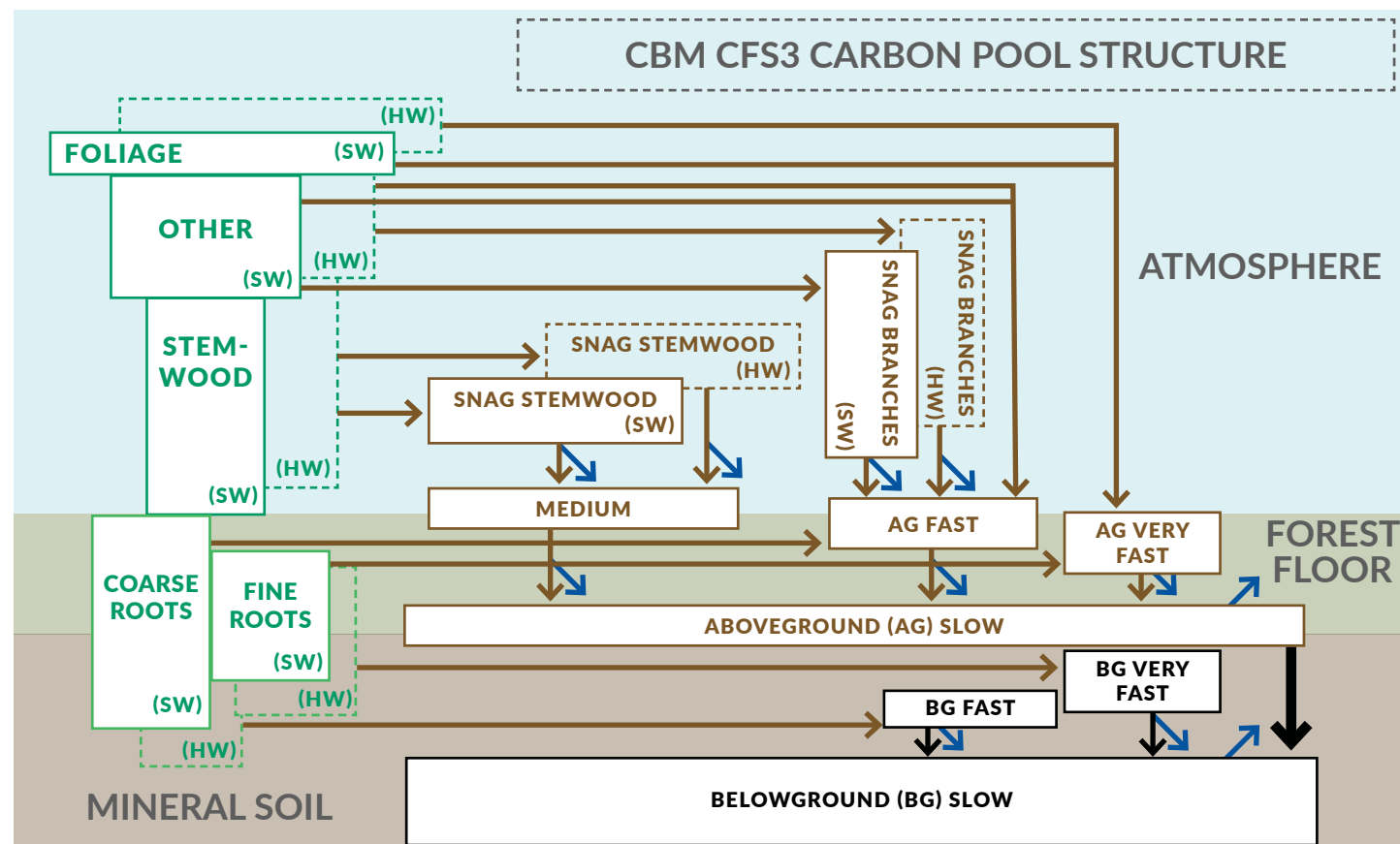
FIGURE 11. CBM-CFS3 CARBON POOLS AND FLOW
